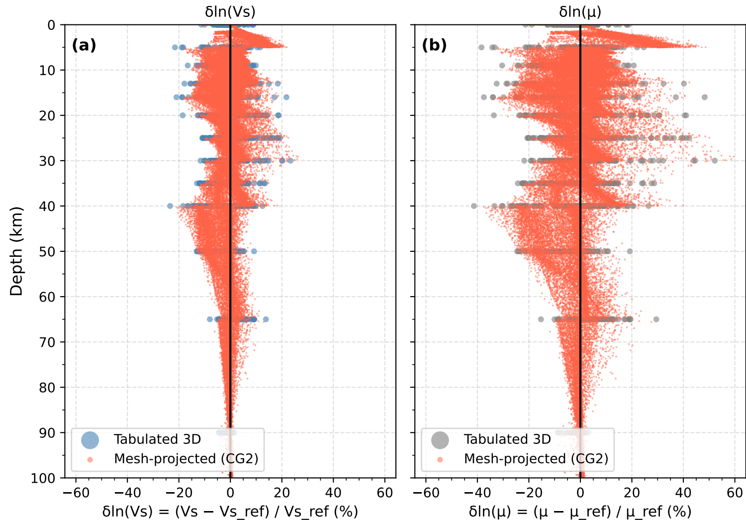
Tabulated 3D vs mesh-projected \delta\ln (hull region, CG2, unscaled)
