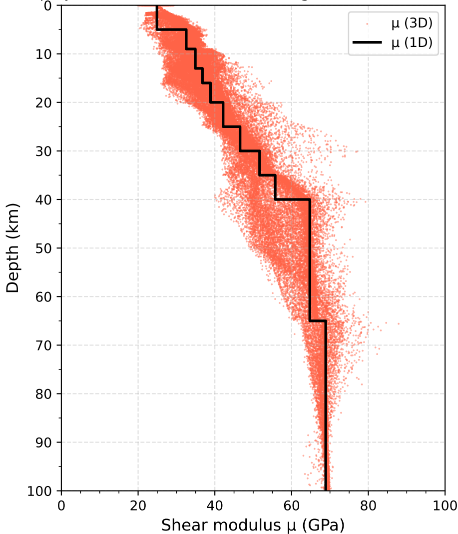
Mesh-projected shear modulus (hull region of 3D, CG2, unscaled)
