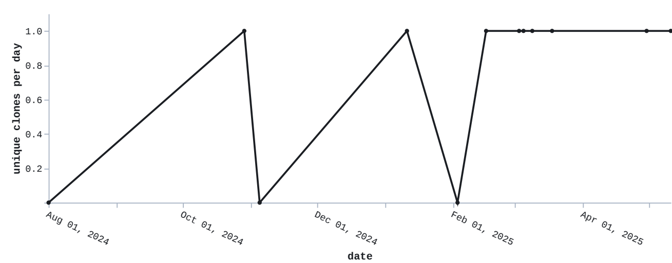
Unique cloners
