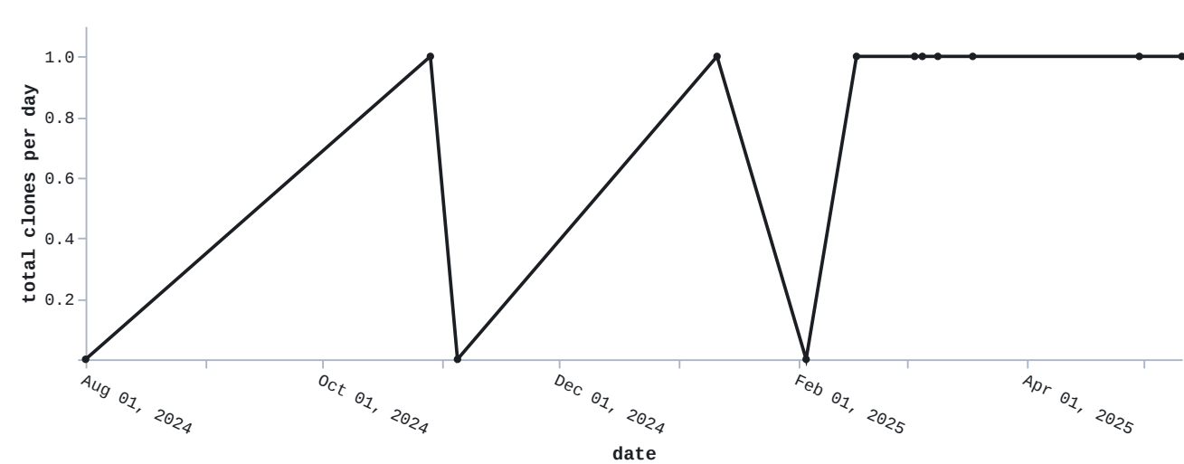
Total clones
