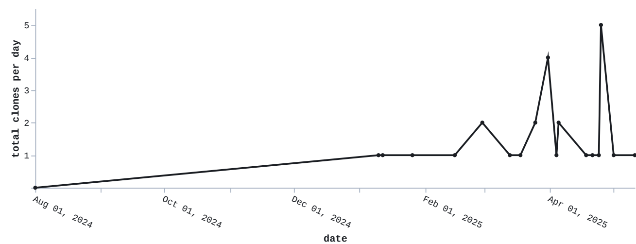
Total clones
