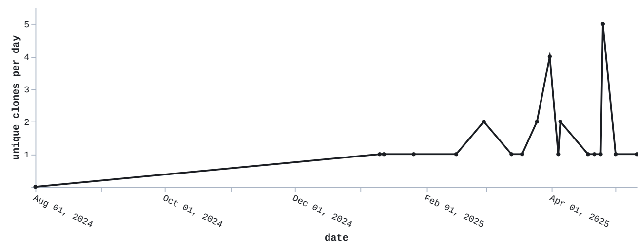
Unique cloners
