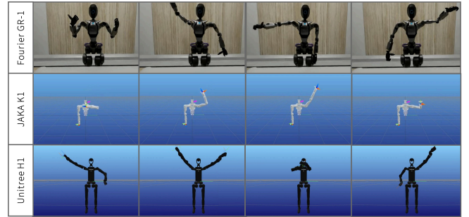
Fig. 6. Cross-platform retargeting on Fourier GR-I, JAKA K1, and Unitree H1 using identical parameters.
