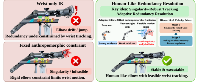
Fig. 1. Human-like redundancy resolution. Wrist-only inverse kinematics leaves the elbow unconstrained, whereas a fixed anthropomorphic objective can become unreliable near full extension. Our method adapts elbow evidence and combines it with singularity-robust wrist tracking.
