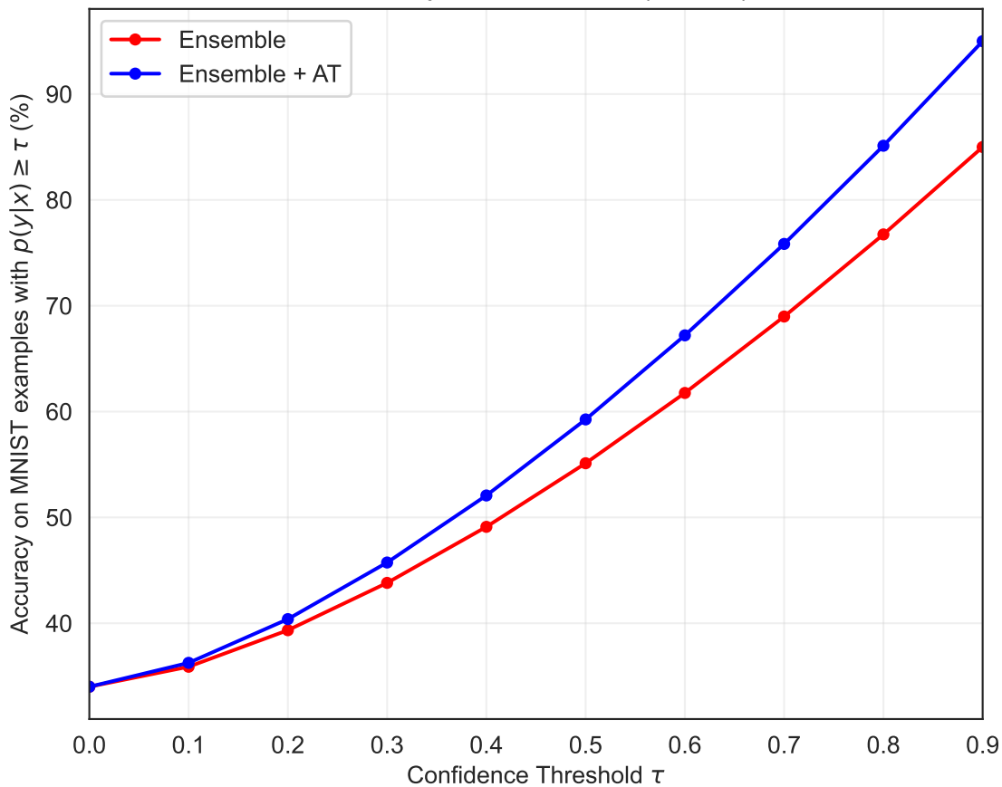
Accuracy vs Confidence (MNIST)
