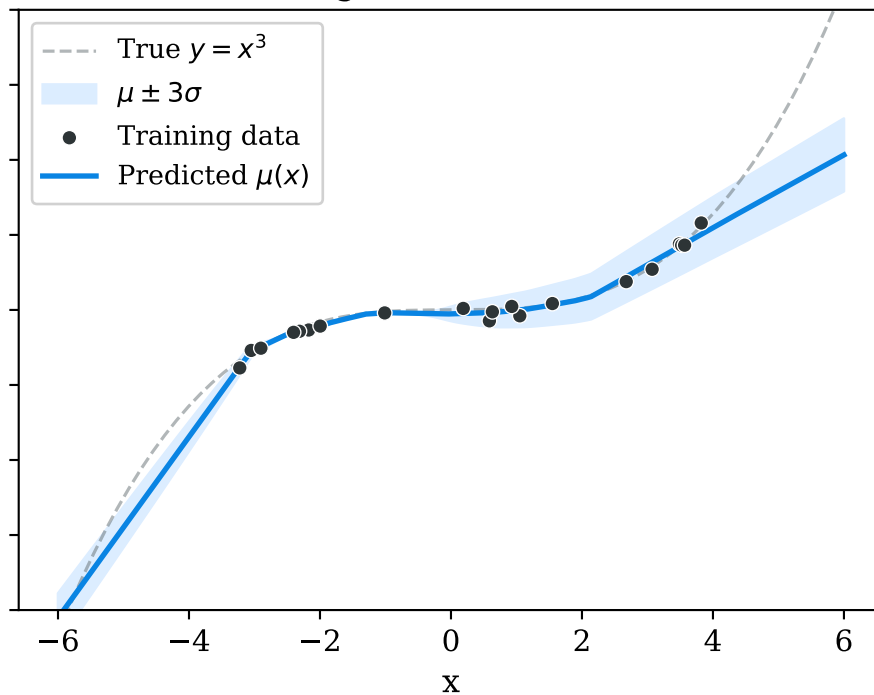
(b) Single NN — NLL Loss
