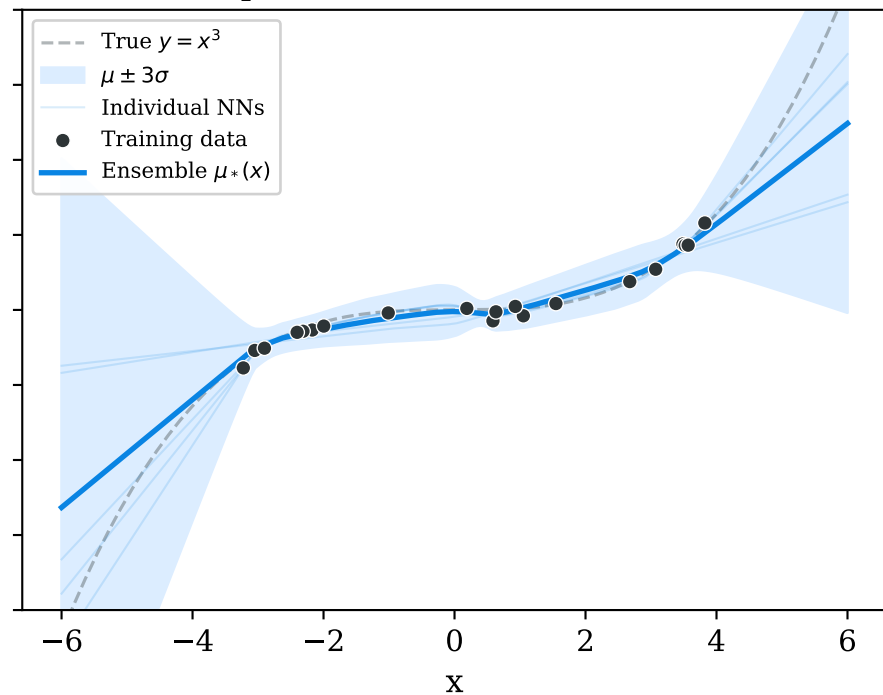
(c) Deep Ensemble (M=5) — NLL Loss
