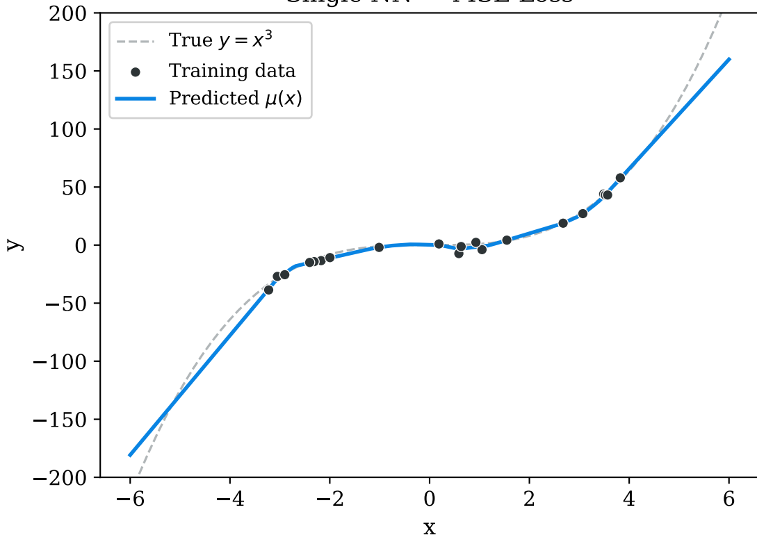
Single NN — MSE Loss
