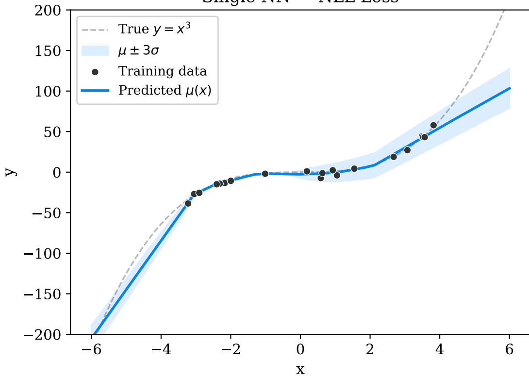
Single NN — NLL Loss
