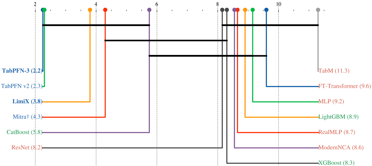
CD diagram — open-source tasks (Friedman \chi^2=138.94 , p=0.0000 )
