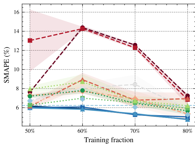
Matbench YS
