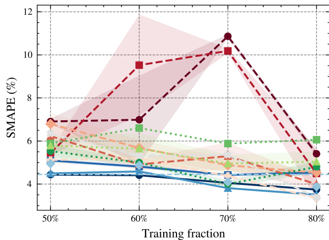
Matbench YS
