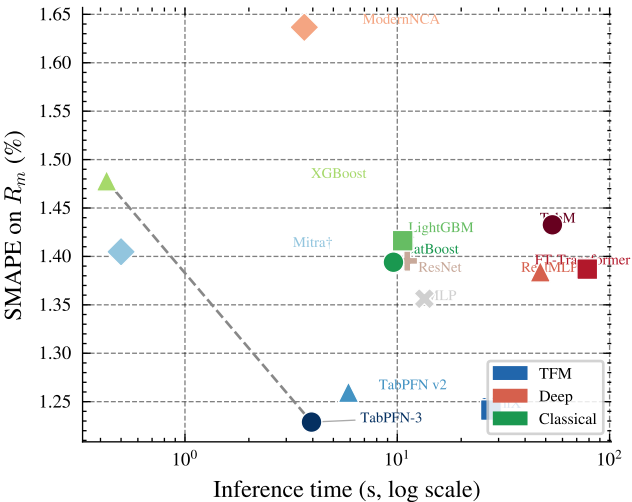
Accuracy vs efficiency ( R_m , 70%)
