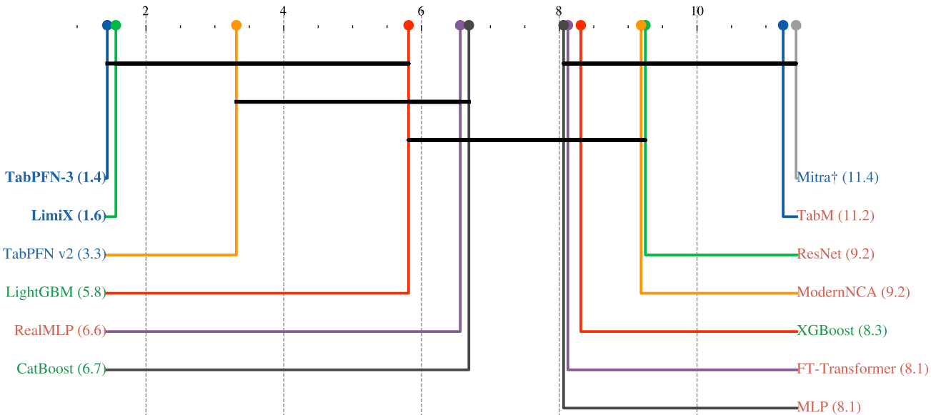
CD diagram — industrial tasks (Friedman \chi^2=134.53 , p=0.0000 )
