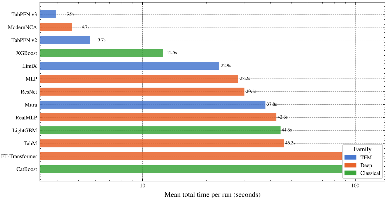
Training + inference time at 70% training fraction (averaged across all datasets)
