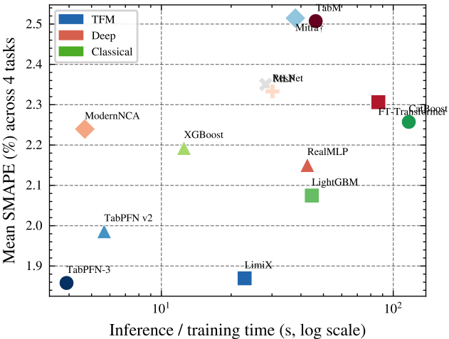
Accuracy–efficiency frontier at 70% training fraction
