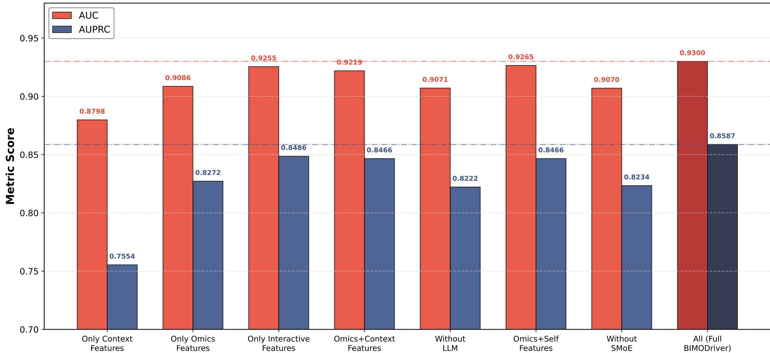
Figure 3: Ablation Study - Component Breakdown (AUC & AUPRC)
