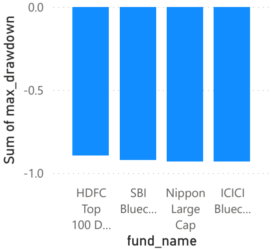
Maximum Drawdown Comparison
