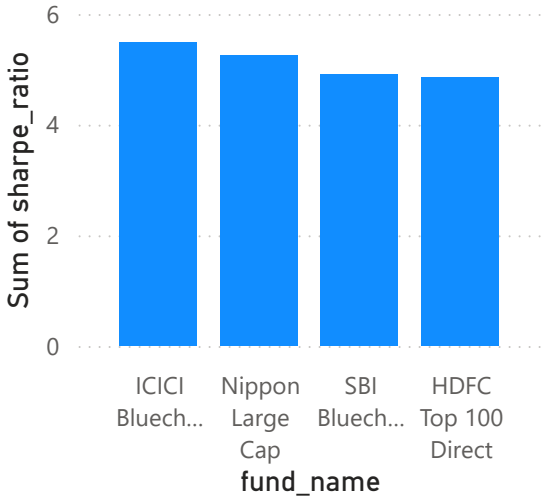
Sharpe Ratio Comparison
