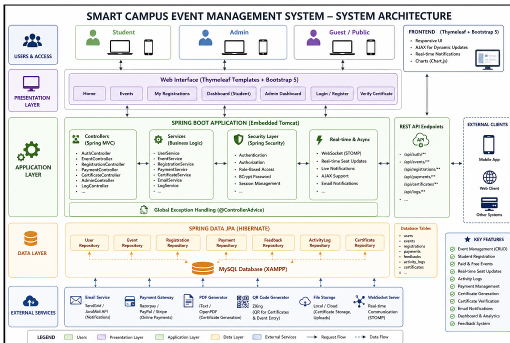
Figure 3.1: Backend Architecture Diagram
