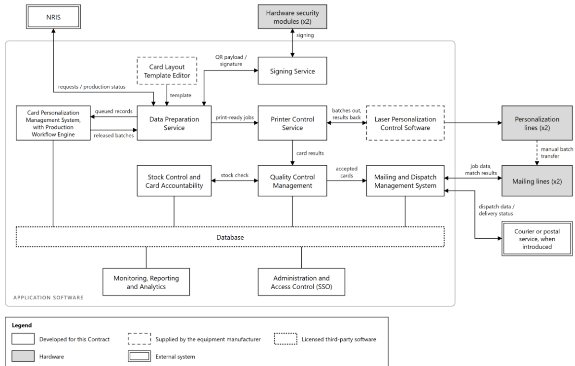
Figure 6.1: Application component architecture. Border style shows ownership; shaded boxes are hardware.
