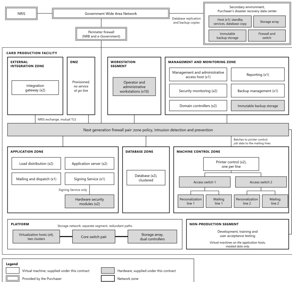
Figure 9.1: Network zones. Every path between zones passes through the firewall pair. Double borders are provided by the Purchaser; shaded boxes are hardware.
