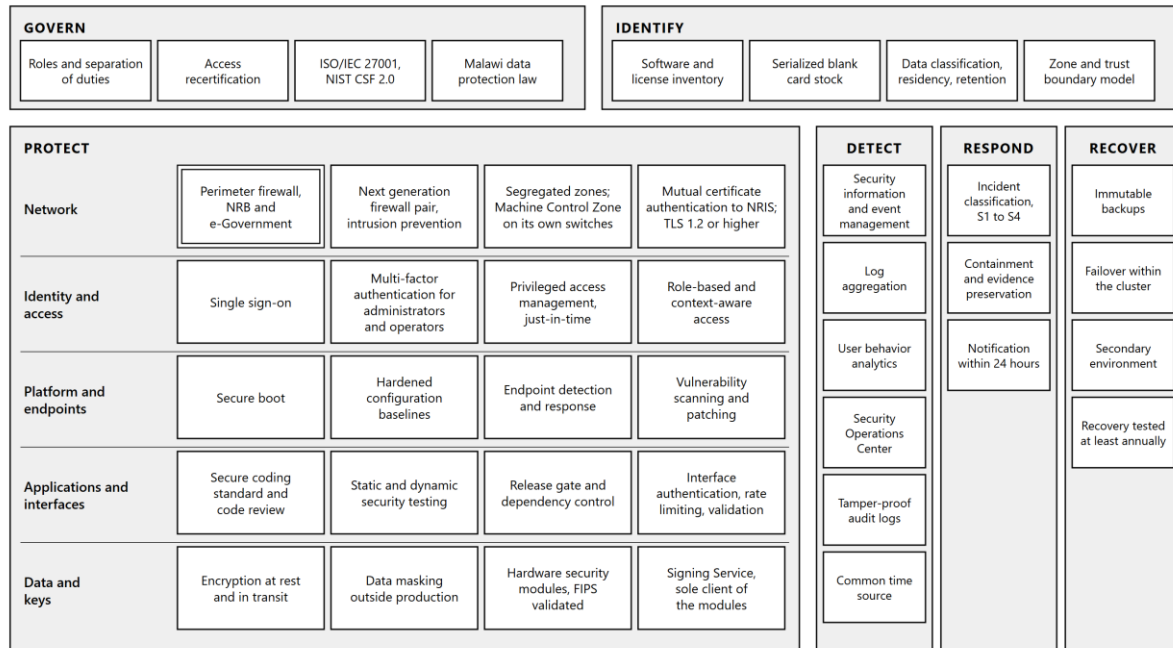
Figure 10.1: Cybersecurity architecture. Protective controls in depth from the network to the data and keys, with detection, response and recovery spanning every layer, arranged by the functions of the NIST Cybersecurity Framework 2.0. The double border is provided by the Purchaser.
