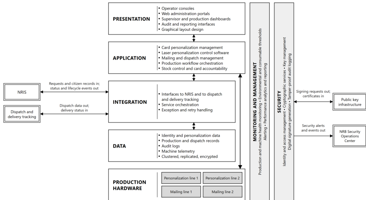
Figure 2.1: Architecture overview. Double borders are external systems; shaded boxes are hardware.
