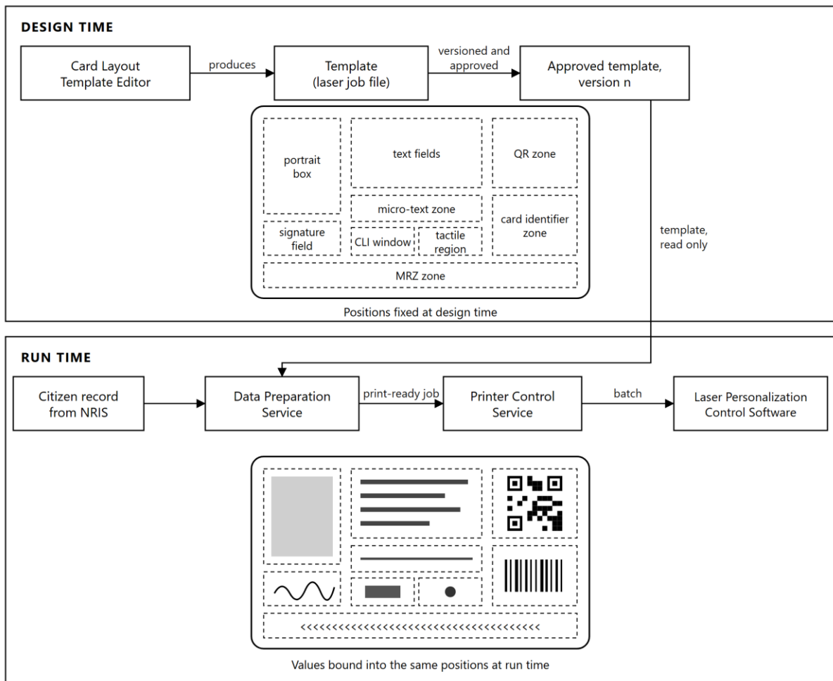
Figure 6.2: Design time and run time. The template fixes the position of every element; the production path binds values into those positions and cannot alter them.
