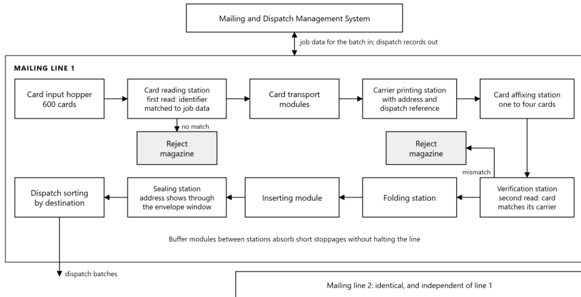
Figure 5.1: Mailing line. Each card is read against the job data before its carrier is printed, and read again with its carrier after affixing, before the mail piece is folded and inserted.
