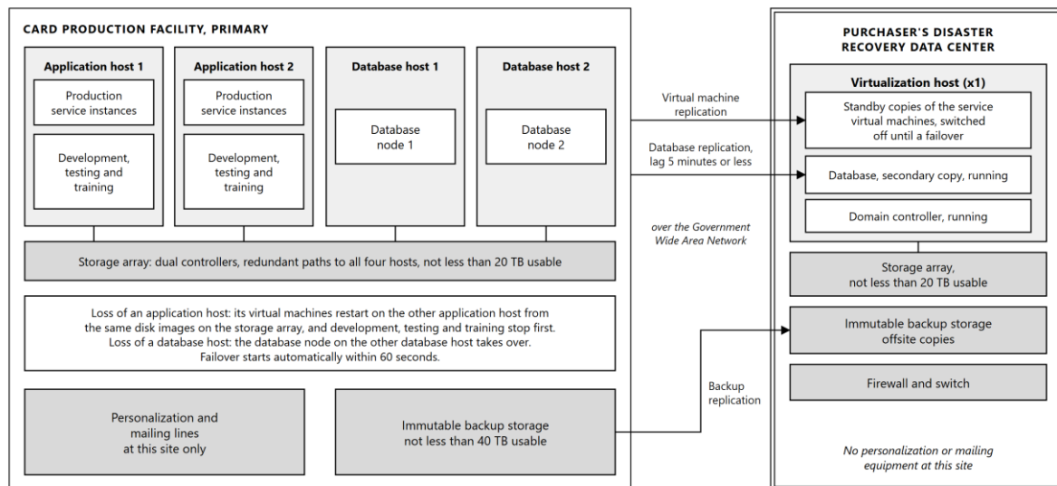
Figure 9.2: High availability and the secondary environment. Double borders are provided by the Purchaser; shaded boxes are hardware.
