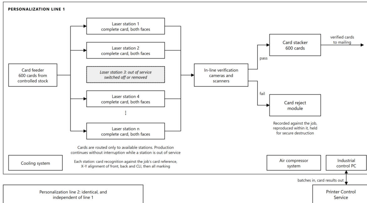
Figure 3.1: Personalization line. Each laser station marks a complete card on both faces; a station out of service is bypassed and production continues without interruption.
