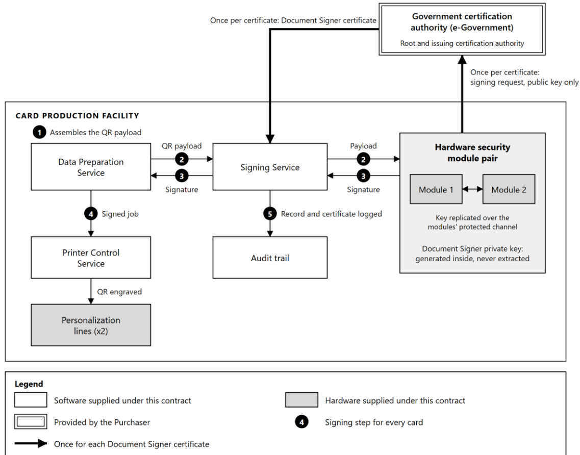
Figure 10.2: Card signing. The Document Signer key is generated inside the hardware security modules and never leaves them; only the signing request and the certificate pass to and from the certification authority. Numbers are the signing steps in the table above.
