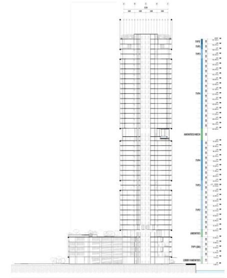
FIG 08.3 Section through the tower and podium.
