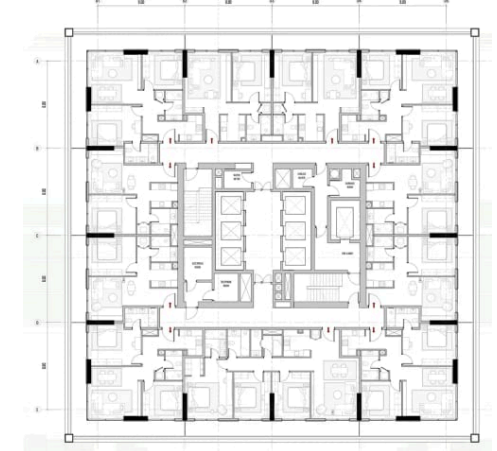
FIG 08.6 Typical floor: the core at the centre, apartments around it.
