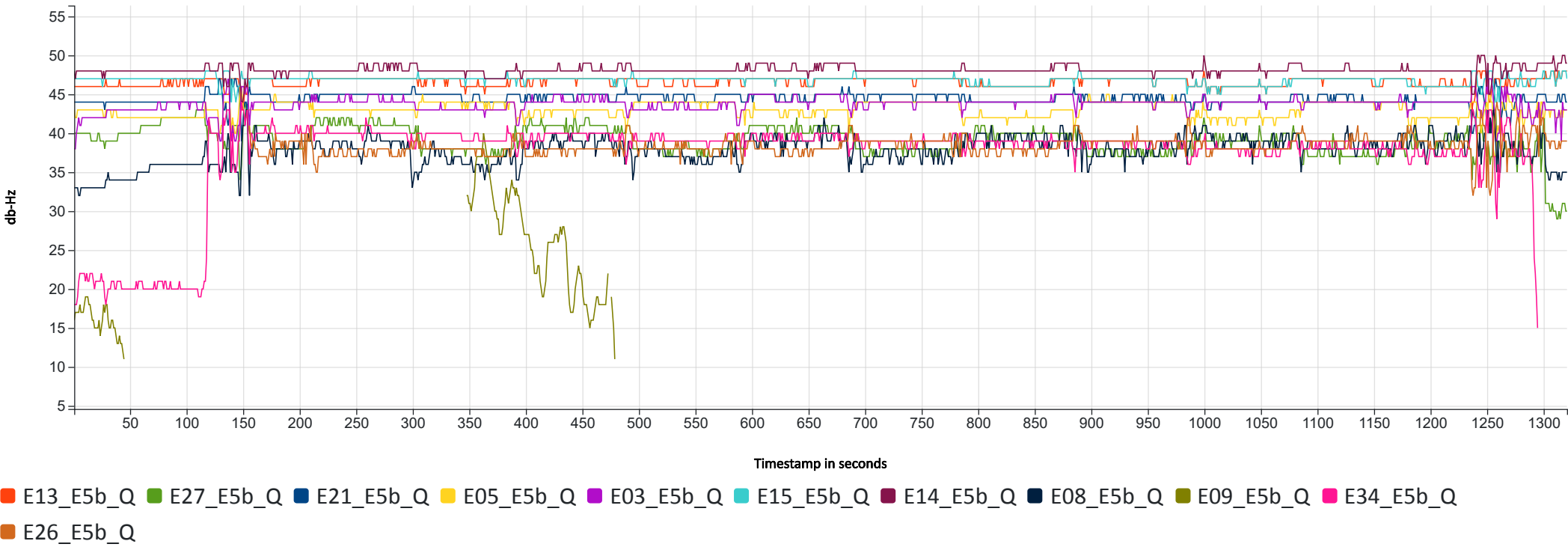
Carrier to noise (dB-hz) - Galileo E5b
