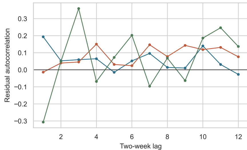
Residual autocorrelation
