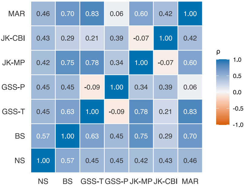
Figure 2: Pairwise Pearson correlations among seven US shock and stance series, common monthly sample 2000-02 to 2014-03. Short labels: NS = Nakamura-Steinsson (2018); BS = Bauer-Swanson (2023) MPS_ORTH; GSS-T and GSS-P = the target and path factors from the Swanson (2021) three-factor decomposition; JK-MP and JK-CBI = Jarociński-Karadi (2020) pure monetary policy and central bank information shocks; MAR = Miranda-Agrippino-Ricco (2021) informationally-robust shock. The diagonal block across the four identified-shock series shows correlations in the 0.4-0.7 range, consistent with Brennan et al. (2024).
