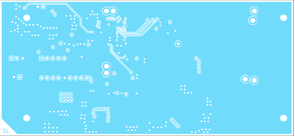
Int2 (GND) (Scale 1:1)
