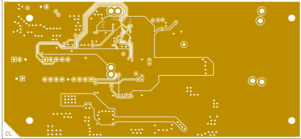
Int1 (PWR) (Scale 1:1)
