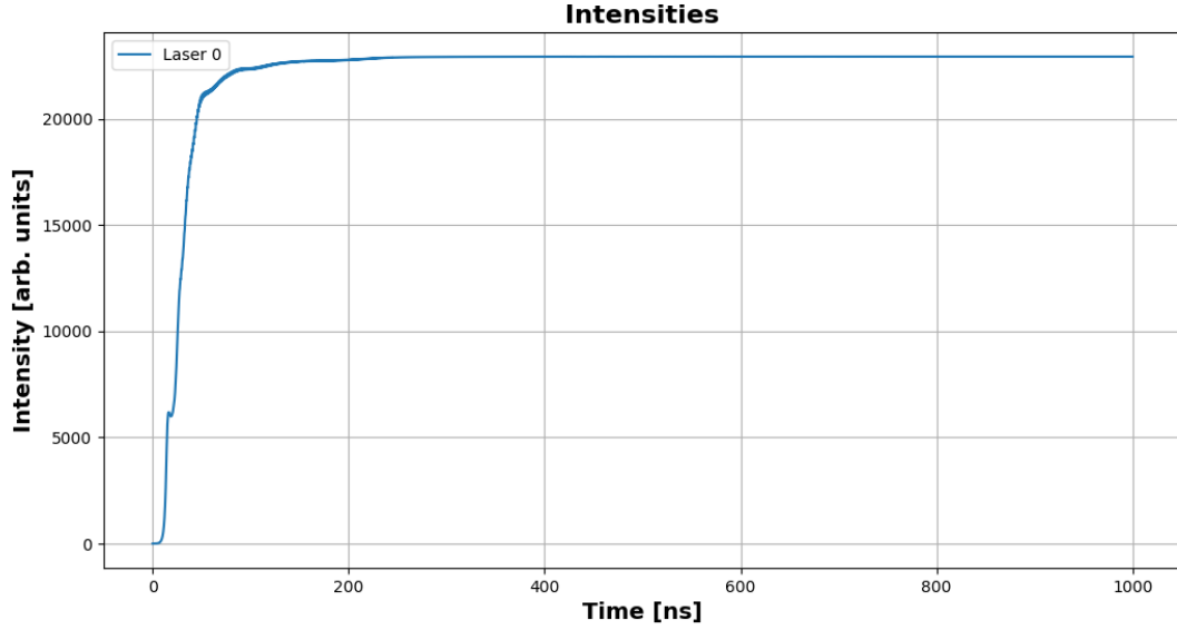
Figure 14: Low-Pass Filtered Intensity for a self-coupled laser w/ \kappa = 0.5 , \tau = 1\text{ns} , driven at threshold current.
