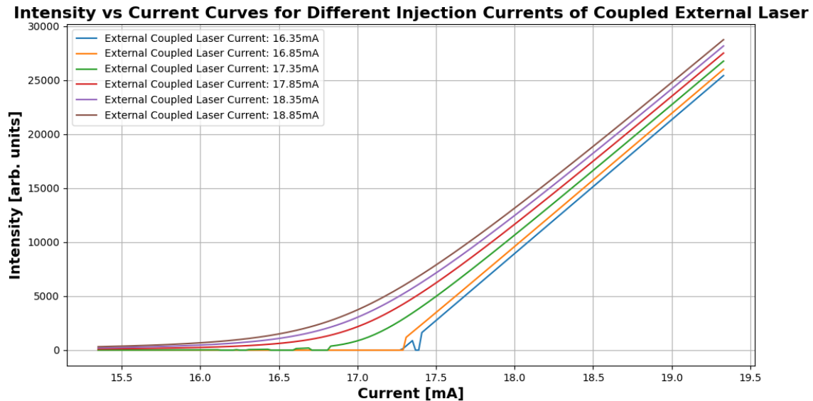
Figure 17: Same graph as 16 except obtained using the steady state solver. Intensity vs. Current curves for a laser coupled to an external laser. Different injection values of the external laser are simulated, which change the curve's characteristics.
