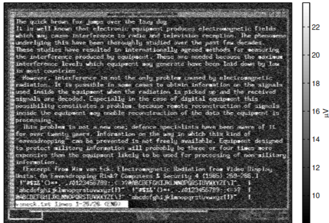
Fig. 3. Text signal received from a 440CDX laptop at 10 m distance through two intermediate offices (3 plasterboard walls). From Kuhn, "Electromagnetic
