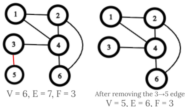
Figure 5: What happens when we remove an edge that is not part of a cycle? (edge 3 \rightarrow 5 )
