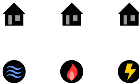
Figure 1: Can you find a way to connect each house to each utility, without any wires crossing?
