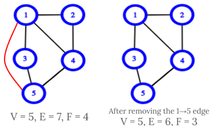
Figure 6: What happens when we remove an edge that is part of a cycle? (edge 1 \rightarrow 5 )
