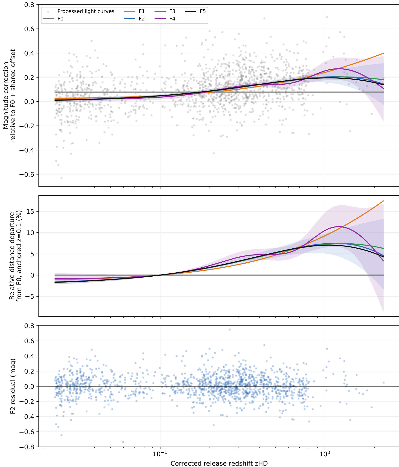
Pantheon+ empirical shape controls — full STAT+SYS covariance DRAFT; no native-law or absolute-distance inference; shaded pointwise 95% bands
