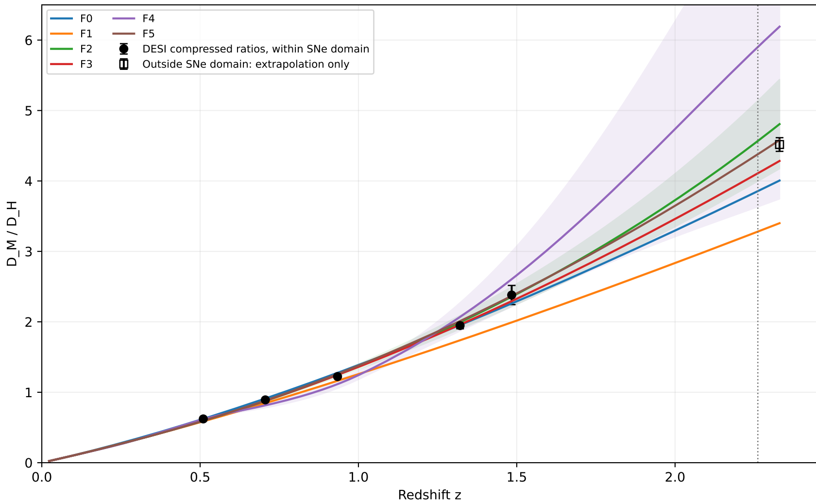
Conditional cross-probe check: SNe-only shapes against BAO Flat homogeneous geometry + conventional ruler/optics; no BAO retuning
