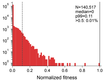
PhoQ
