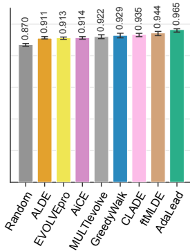
CreiLOV multi-site
