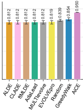
GFP multi-site
