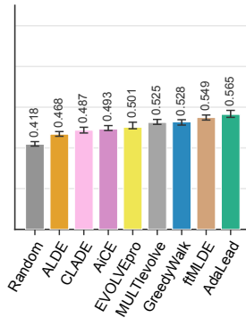
PAB1 multi-site
