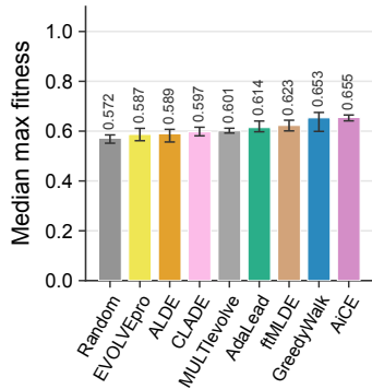
AAV multi-site
