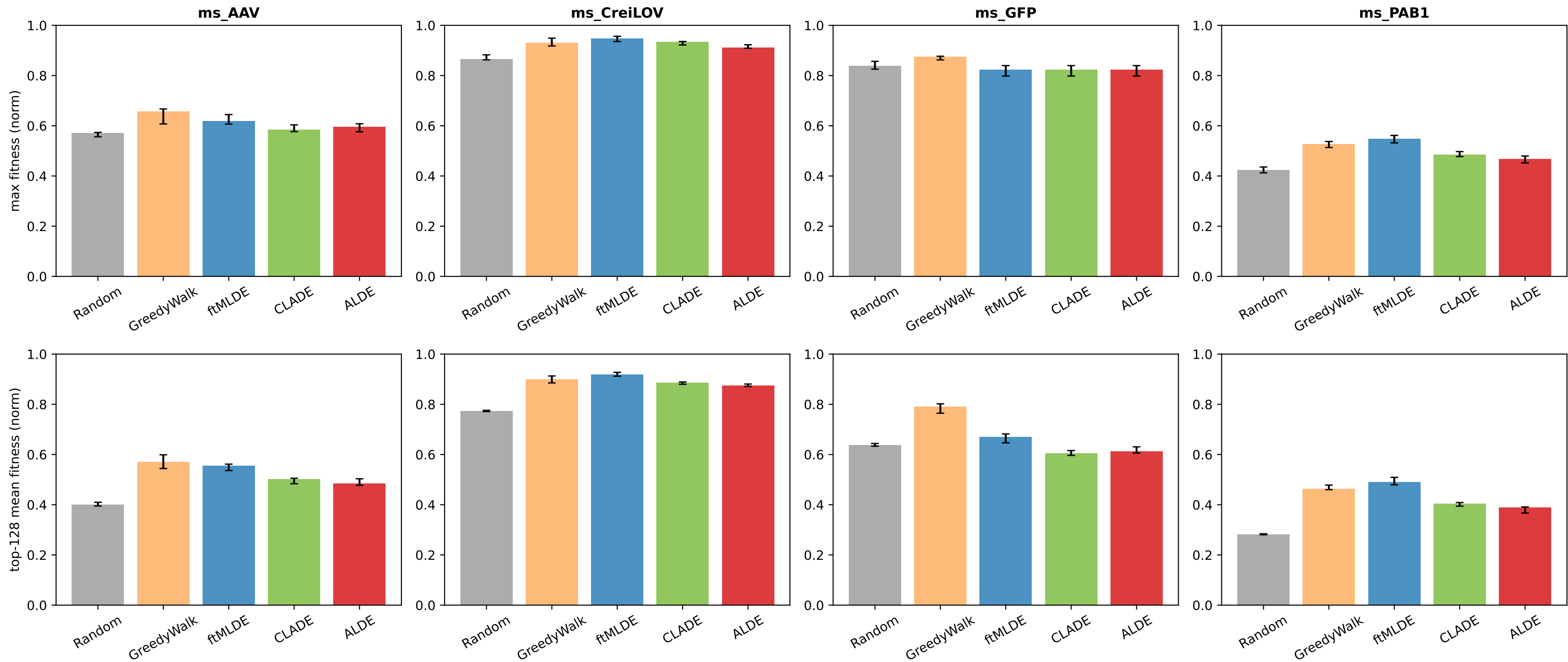
Multi-site oracle benchmark — max fitness (top) and top-128 mean fitness (bottom); median \pm IQR over seeds
