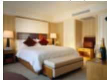
defocus (s5)
