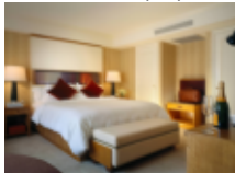
motion (s5)
