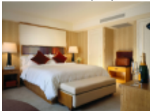
elastic (s3)
