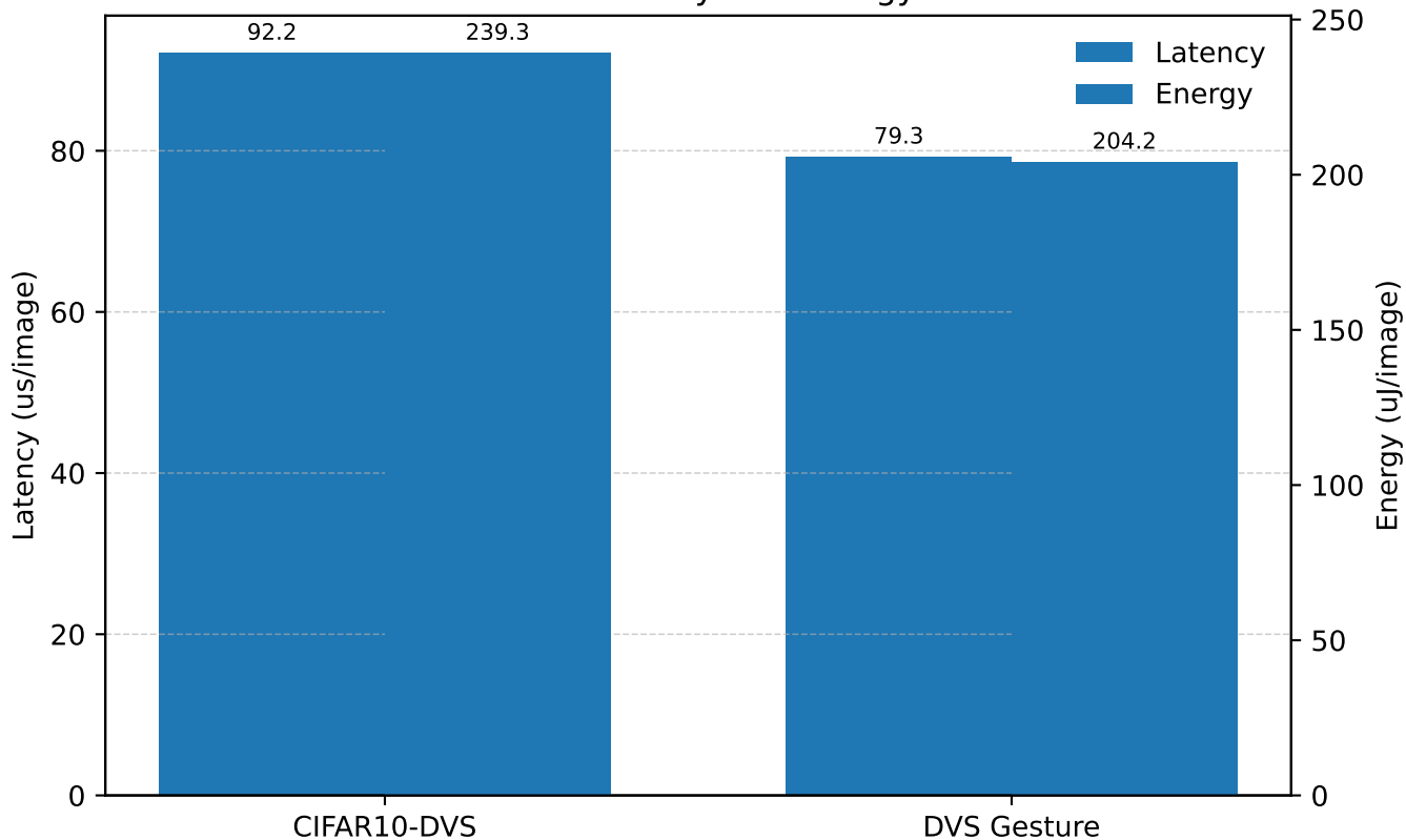
HIPSA latency and energy
