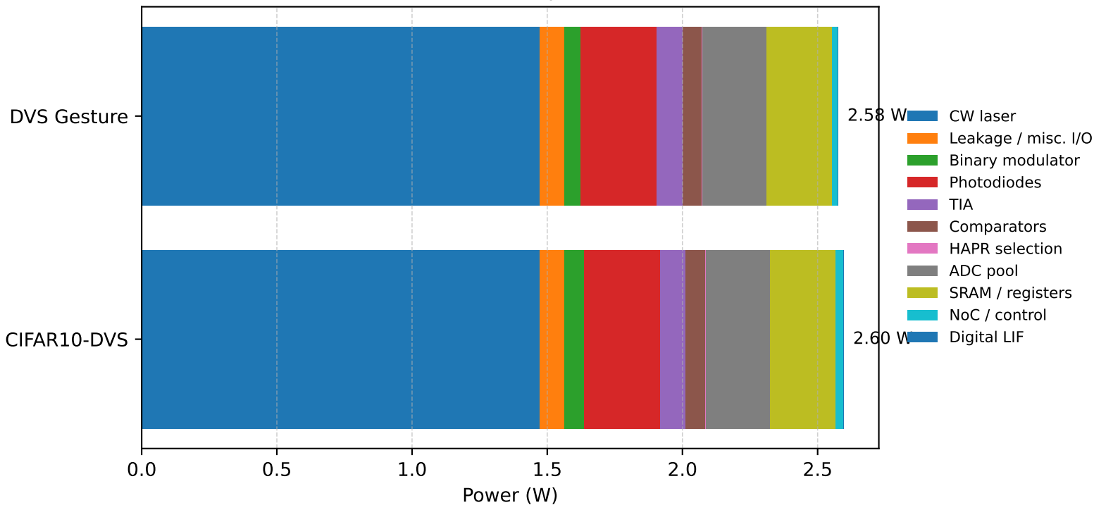
HIPSA device-calibrated power breakdown
