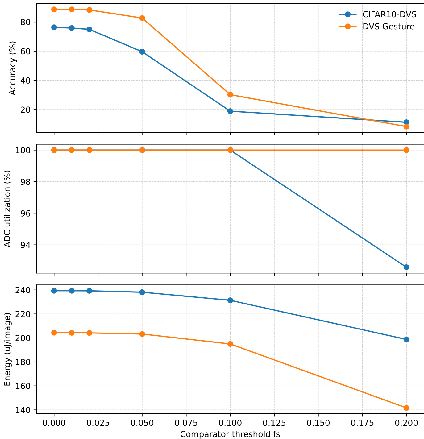
Comparator threshold sweep
