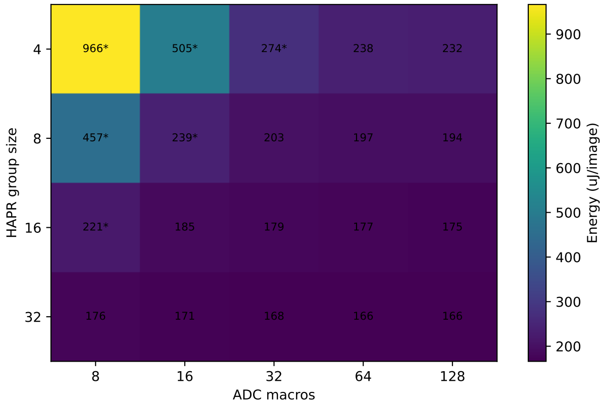
HAPR / ADC energy sensitivity: CIFAR10-DVS
