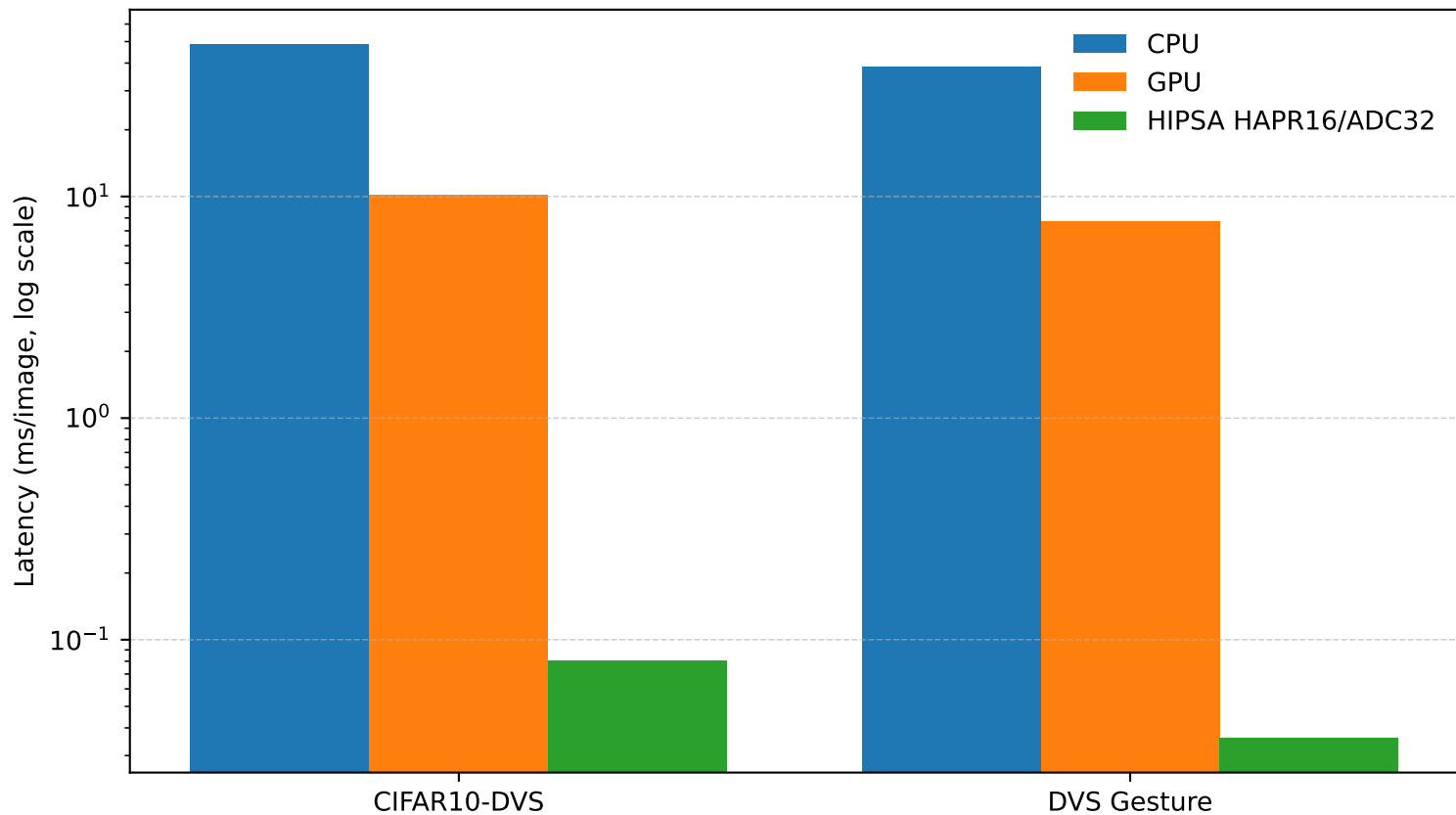
Software baseline vs HIPSA
