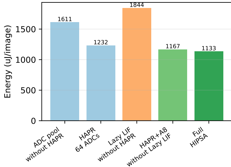
DVSGESTURE
