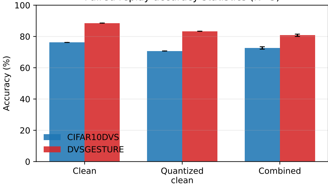
Paired replay accuracy statistics (N=5)
