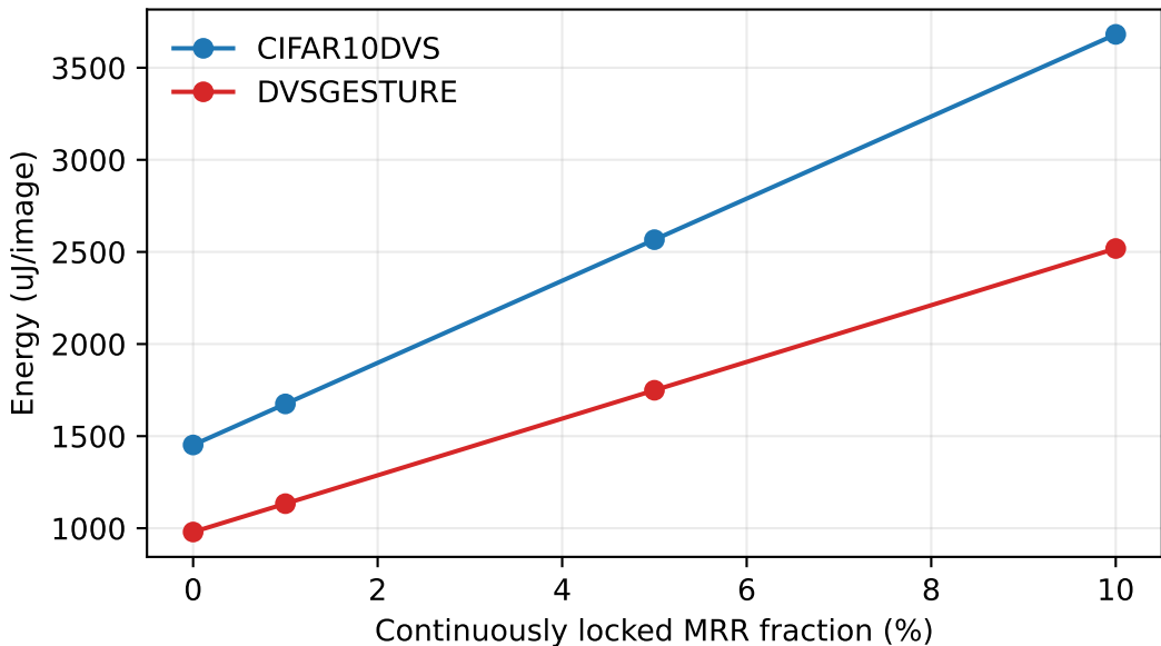
Parameterized MRR lock-power sensitivity
