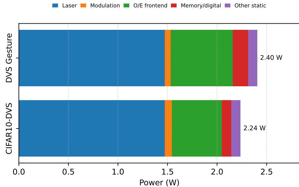
(a) Balanced power breakdown
