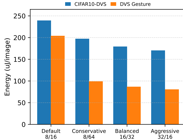
(b) HAPR/ADC energy
