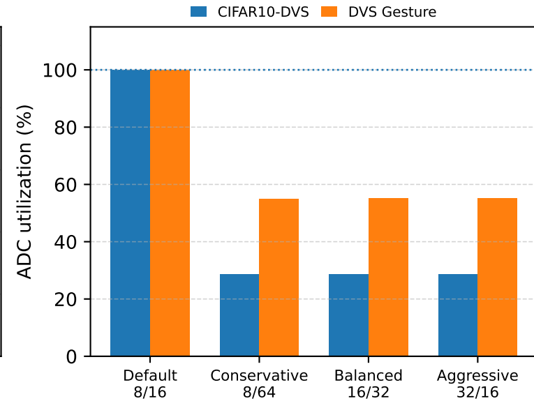
(c) ADC backend pressure
