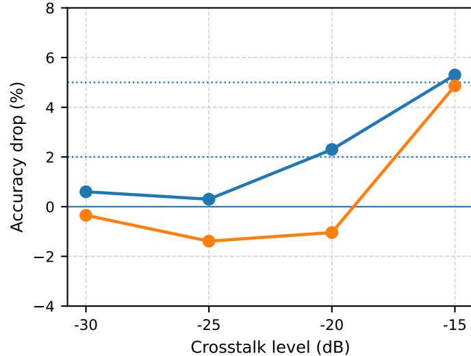
WDM crosstalk
