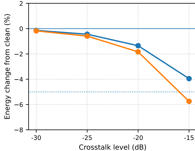
WDM crosstalk
