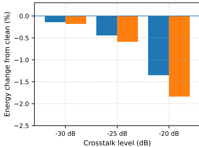
WDM crosstalk
