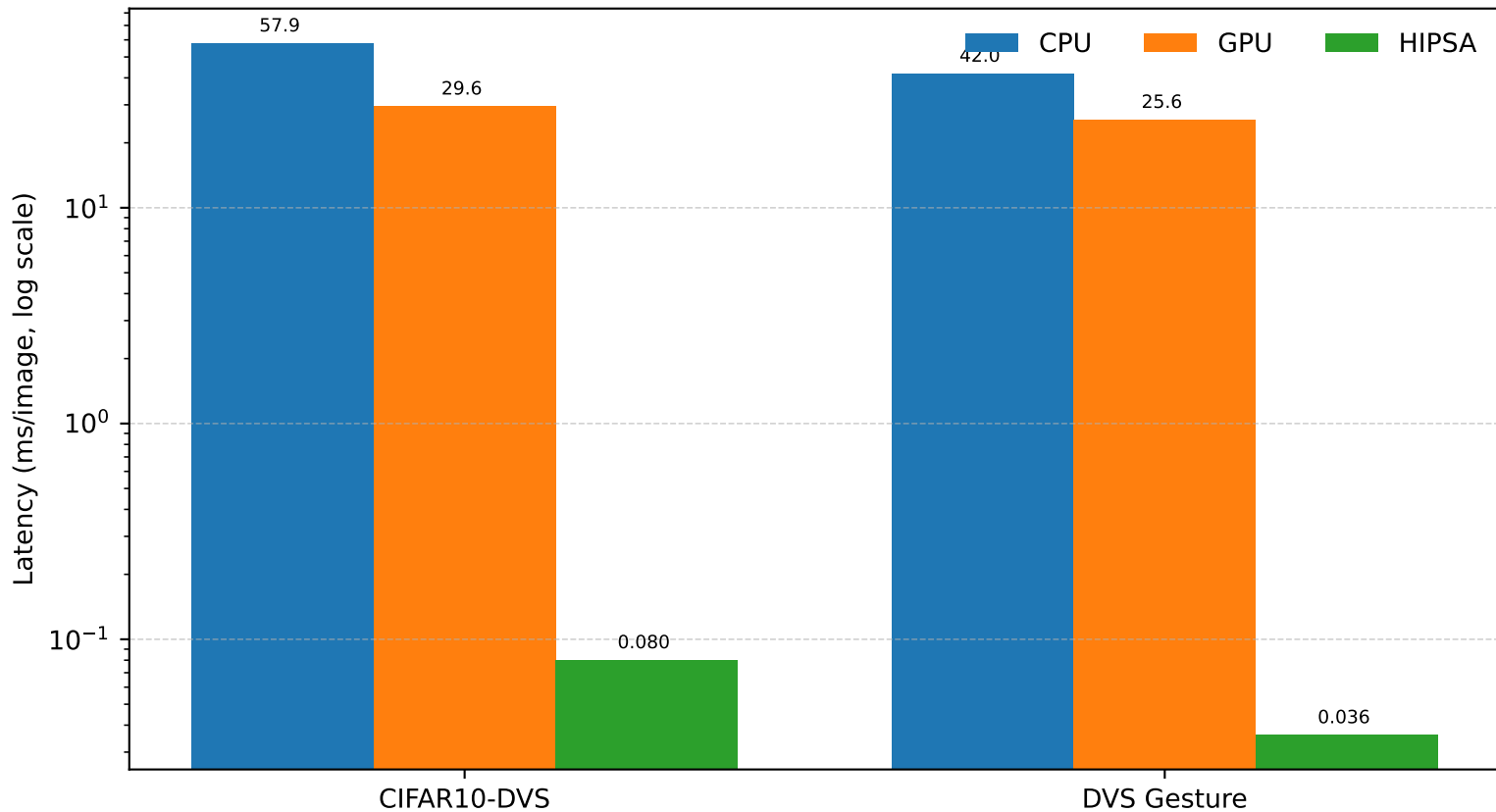
CPU/GPU/HIPSA latency comparison
