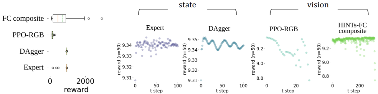
Figure 7. Inverted Double Pendulum reward corresponding to results reported in Tab 2 ( n=50 seeds). (Left) HINTs-FC outperforms PPO-RGB while approaching DAGGER. (Right) Instantaneous reward vs trajectory time step.
