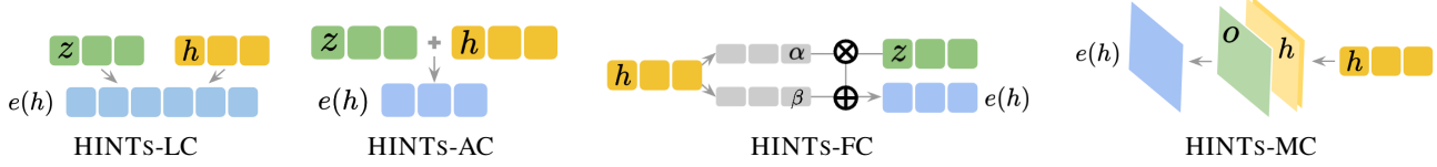
Figure 6. Hint conditioning mechanisms. Agents take image inputs and grounded hints generated by G_\phi and output continuous actions. The inputs are processed by an image encoder and hint a encoder which produce z and h . A conditioning mechanism e to yields inputs to the actor and critic networks from z and h . The conditioning scheme may be task dependent. For example, tasks in which the dimensionality of cues is dominated, e.g., d \ll k , conditioning at the input may preserve hint signal better than conditioning in the latent space.
