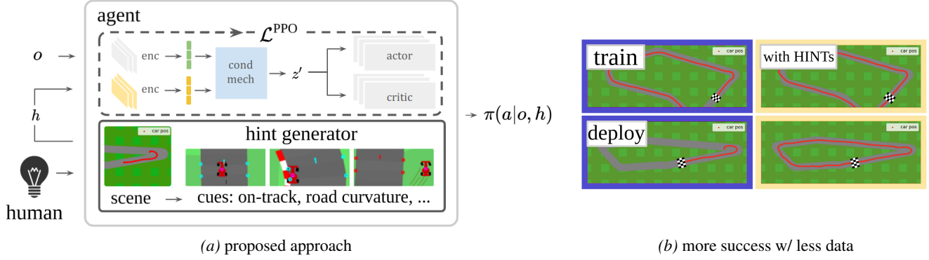
Figure 1. Our proposed framework, HINTS, addresses RL for continuous control in partially observable environments. It allows humans to coach agents while they learn from a limited number of training episodes. a) A generator G_\phi (left) outputs learnt human-intuited cues h (e.g., interpreted as the road curvature) on which policies condition their actions ;-e.g., the road curvature (Sec 3.1). b) As a result, hint-conditioned agents learn precise control tasks with a small training budget. For more complex tasks (right), HINTS allows agents to learn more effective policies than those of vanilla agents; e.g., for passing hairpin corners.
