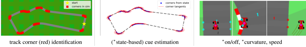
Figure 5. Visualisations of programmatic generation of grounded hints (cues) for Car Racing.
