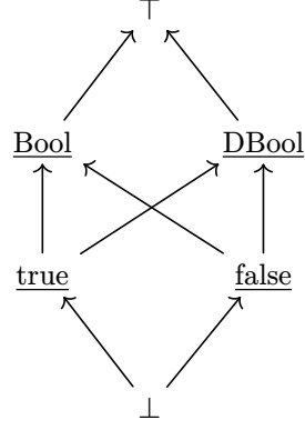
Figure 9: Subtyping lattice for booleans. Arrows denote \sqsubseteq .
