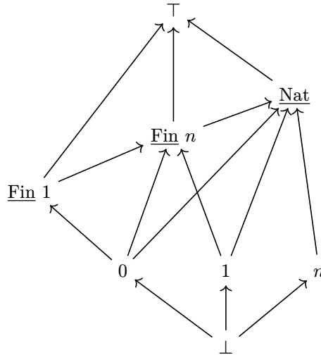
Figure 10: Subtyping lattice for natural numbers and finite sets. Laid out such that subtypes are physically beneath their supertypes.
