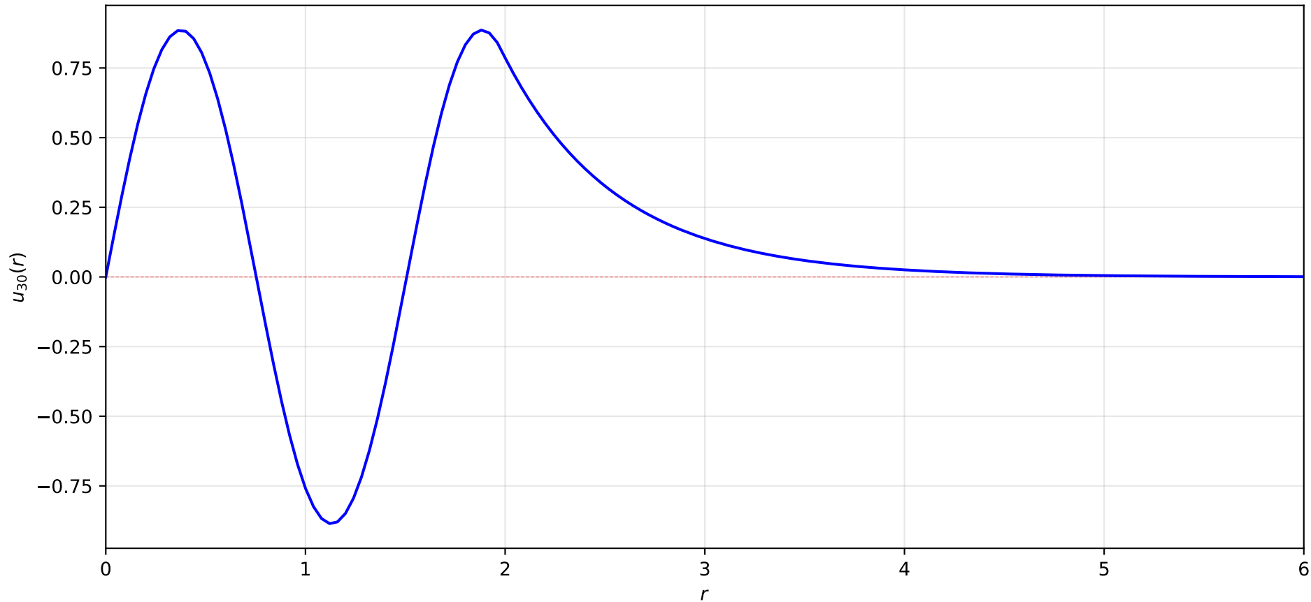
Reduced Radial Wave Function: n = 3, \ell = 0
