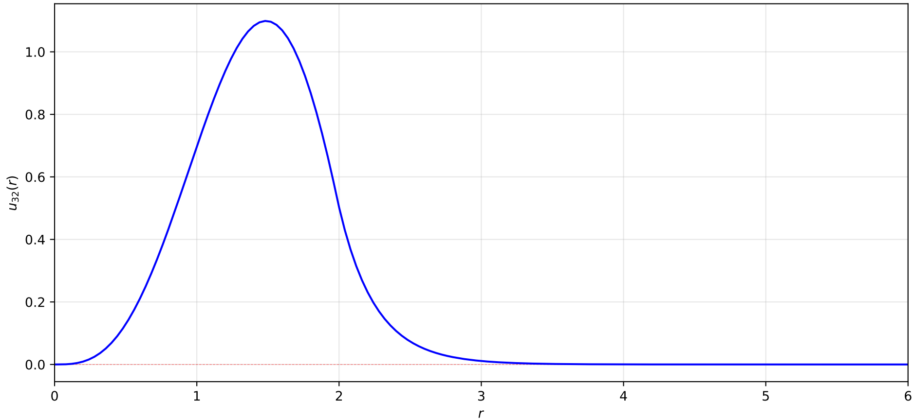
Reduced Radial Wave Function: n = 3, \ell = 2
